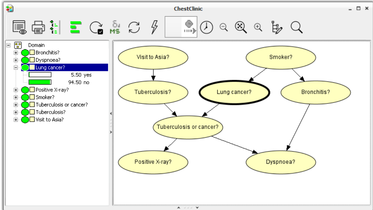
Figure 1: The network window of a HUGIN network running in Run Mode.
