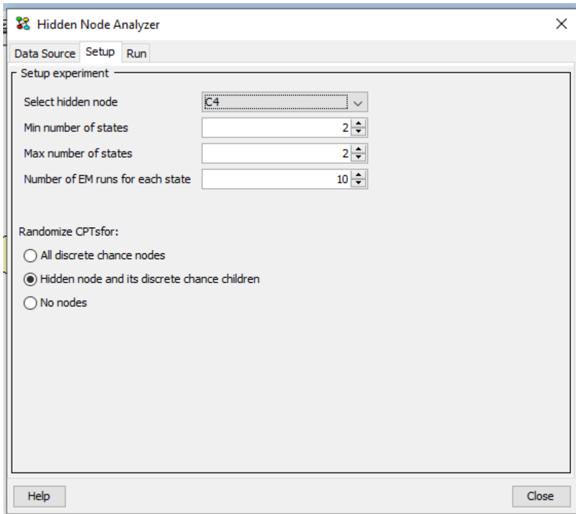
Figure 2: Setup pane.
