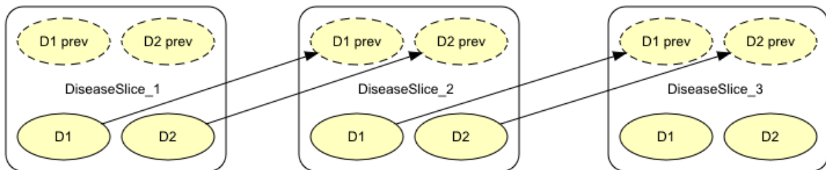
Figure 3: A 3-time slices dynamic Bayesian network (DBN) specified as an object-oriented network.
