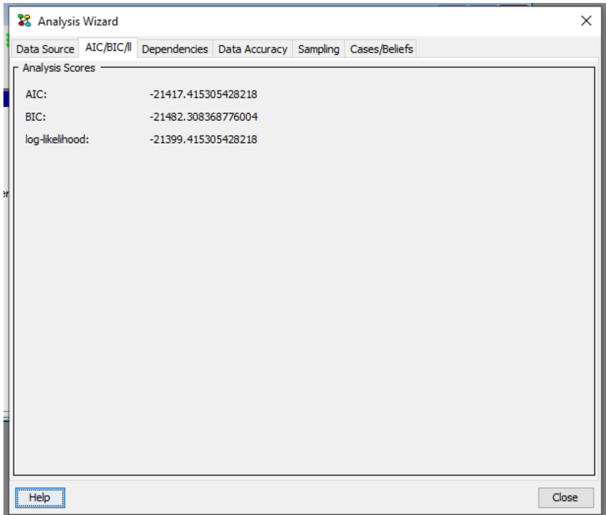
Figure 1: AIC/BIC/ll pane.
