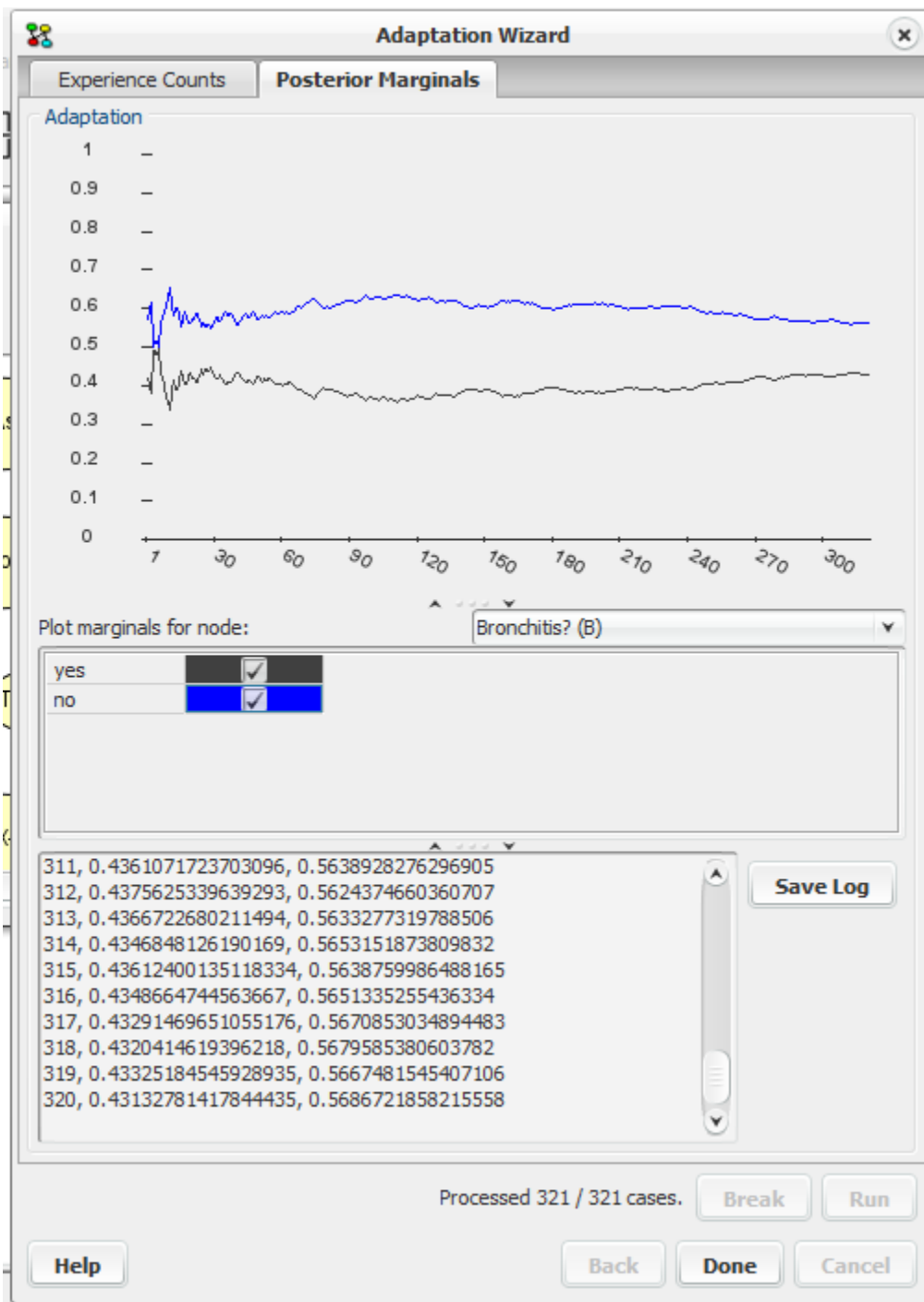
Figure 5: Posterior marginals.
