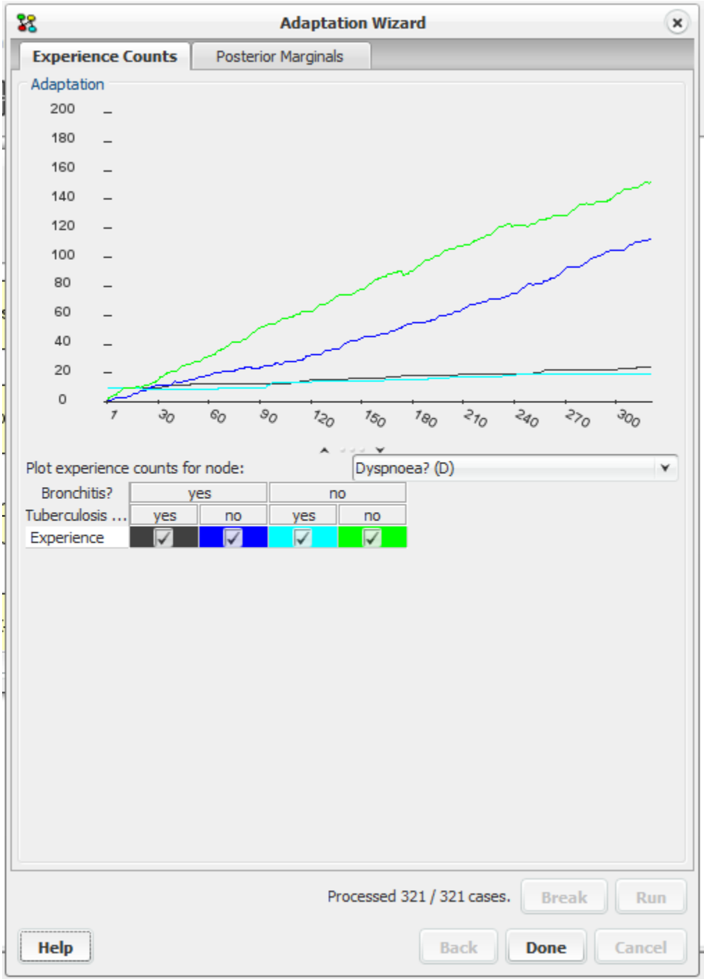
Figure 4: Experience counts.
