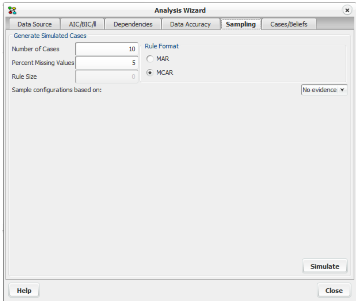
Figure 2: Sampling pane.
