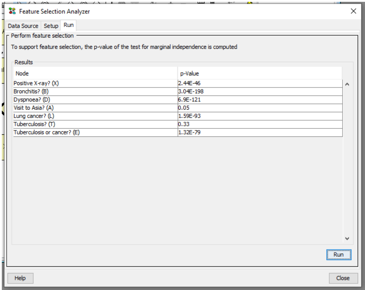
Figure 3: Run Pane.
