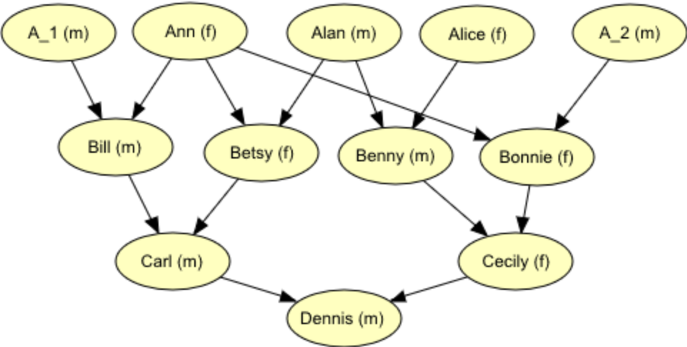
Figure 1: Dennis’s genealogy.
