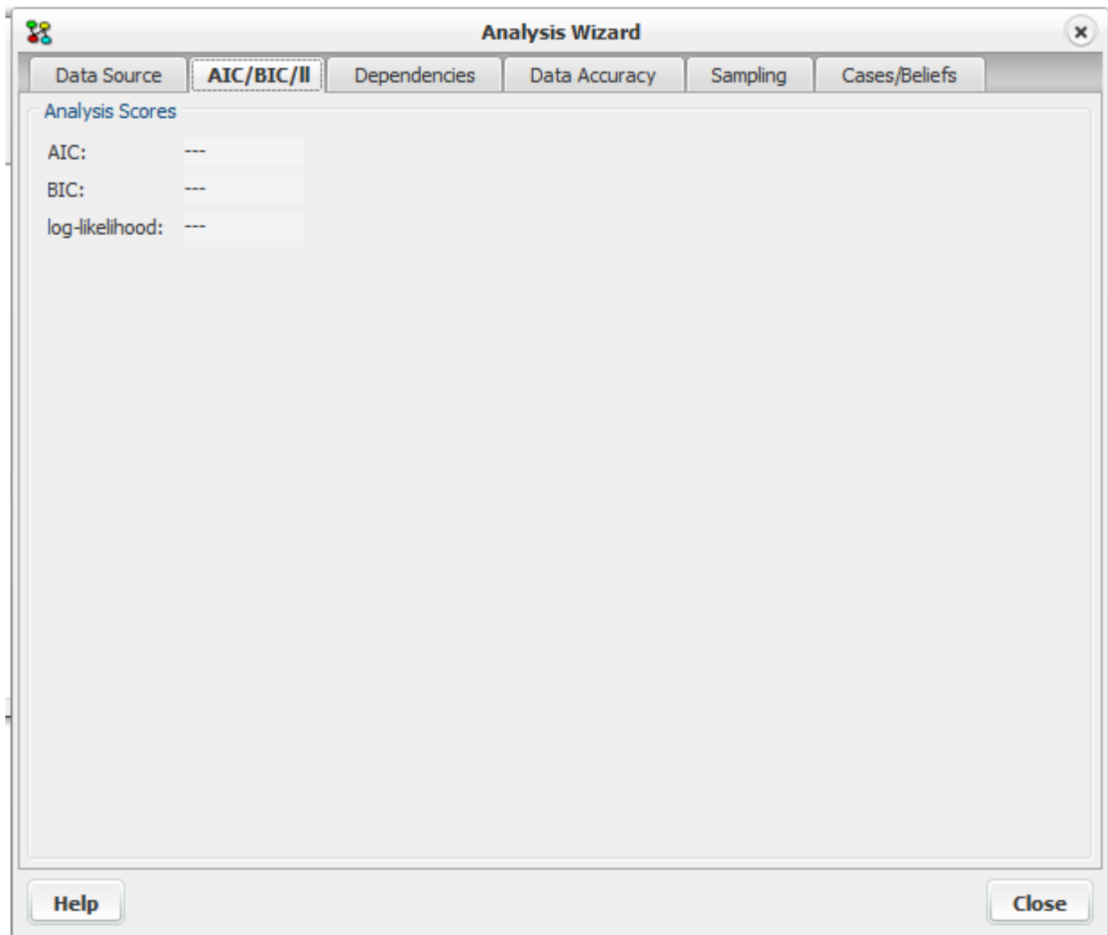
Figure 3: AIC/BIC/II pane.
