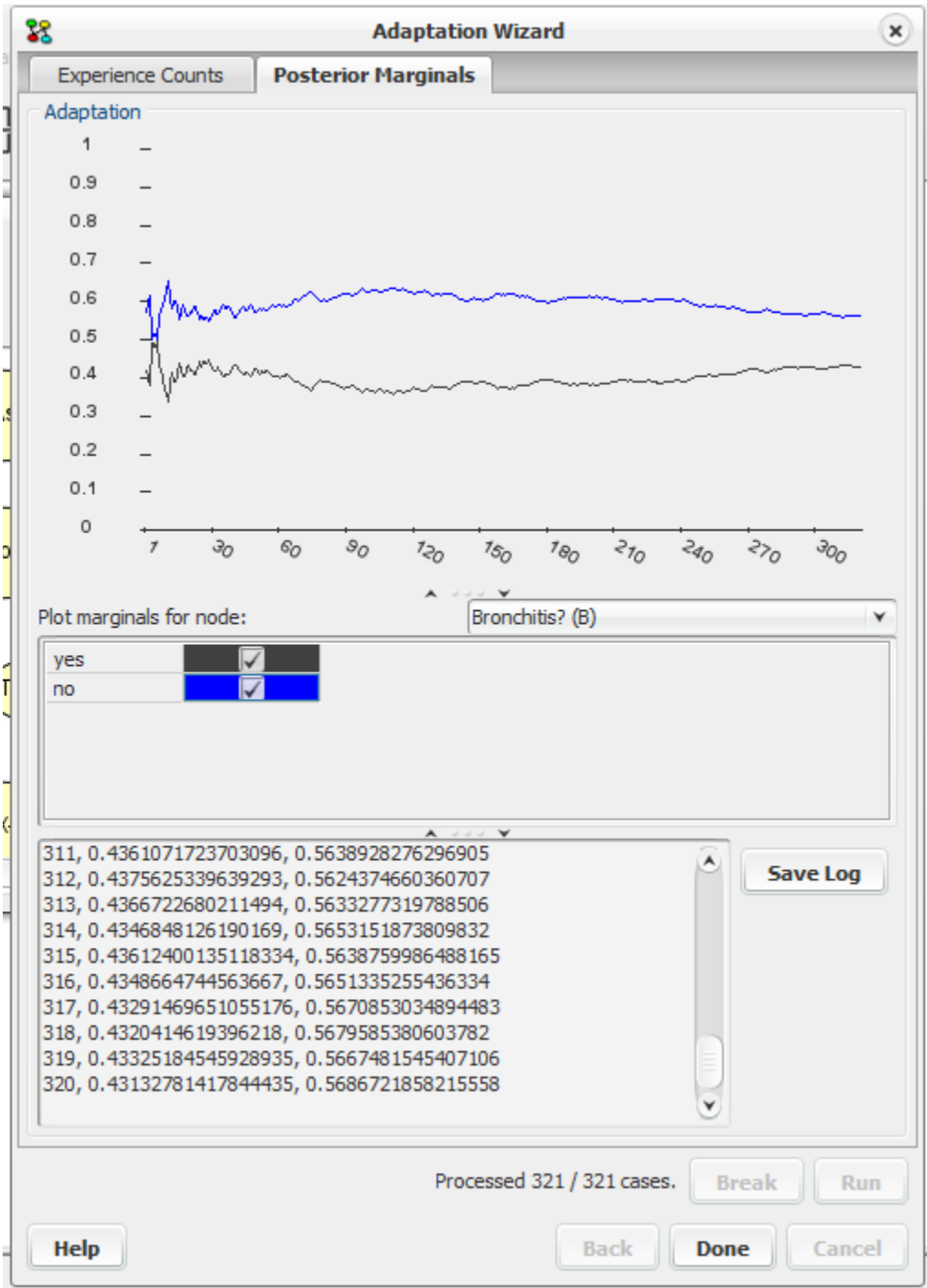
Figure 5: Posterior marginals.
