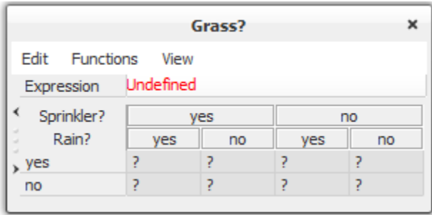
Figure 2: A CPT in expressions mode.
