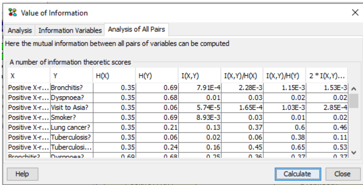
Figure 9: the results of an Analysis of All Pairs calculation.
