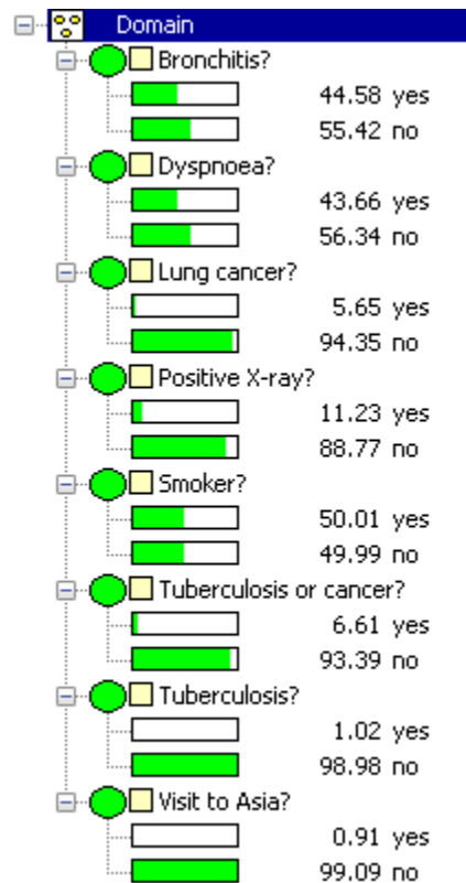
Figure 6: The estimated marginal probability distributions.
