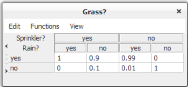
Figure 1: A CPT in manual mode.
