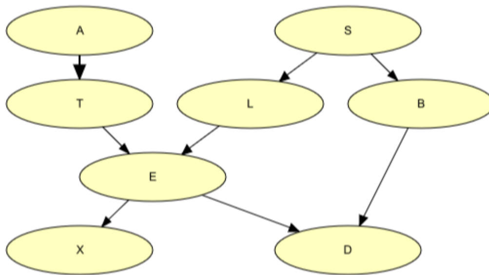
Figure 1: The structure from which the data were sampled.
